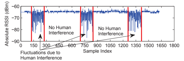
Fig. 2. Absolute RSSI reading
