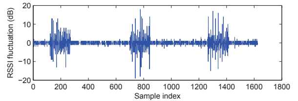
Fig. 3. RSSI Fluctuation
