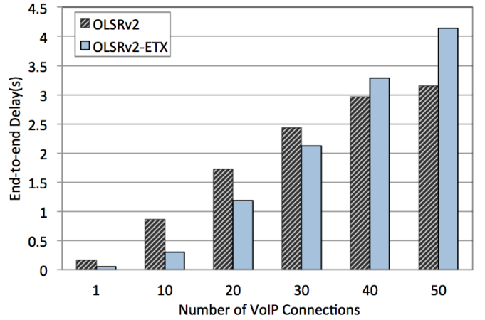
Fig. 2. Average End-to-end Delay
