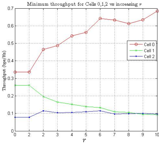
Fig. 7. Throughput in Cells 0 to 2 vs r
