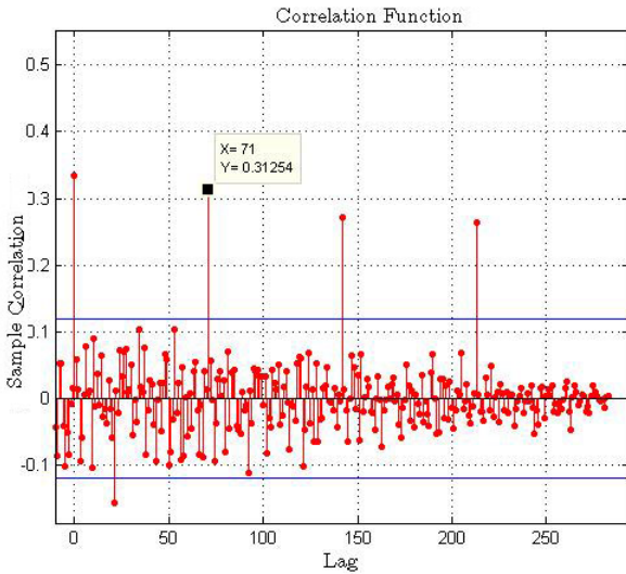
Fig. 4. Auto-correlation plot of a preamble of length 284 bits made with 4 repeated sequences of length 71.
