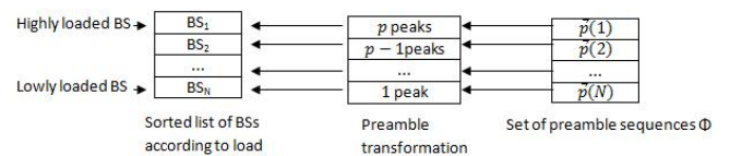
Fig. 2. At central controller the metric is number of peaks in the auto-correlation plot.
