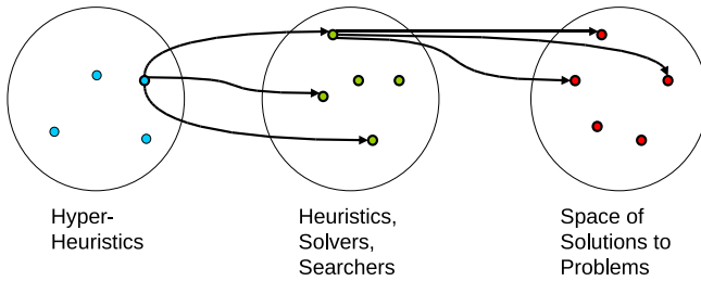
Fig. 1. A hyper-heuristic exploring the space of search algorithms (or more generally solvers) for a particular problem
